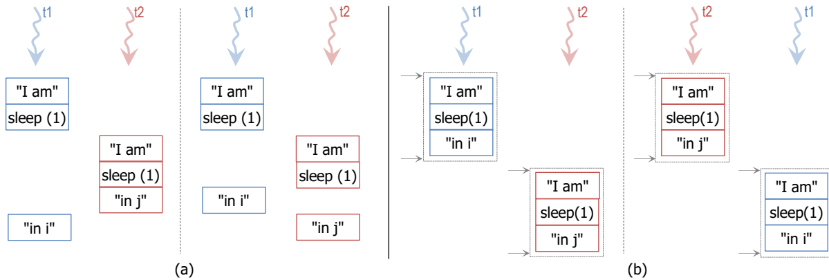
Figure 5. (a) Two execution samples without mutex. (b) Two execution samples with a mutex.
