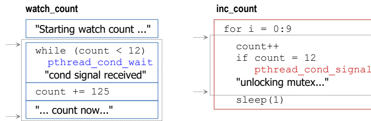
Figure 7. Functions representing the operations of each thread (watch_count: t1, inc_count: t2, t3). Note the mutex lock/unlock. Also note which function issues the signaling and which is waiting for the signal (when the condition is met)
