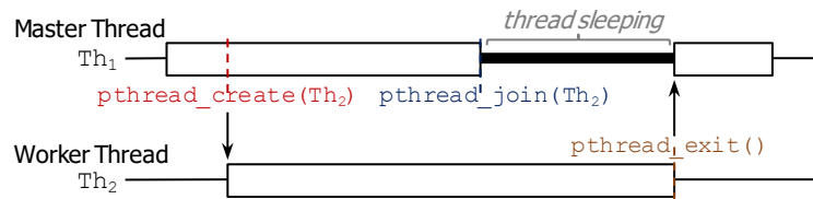
Figure 2. Master thread creates and joins a thread that uses pthread_exit to exit.
