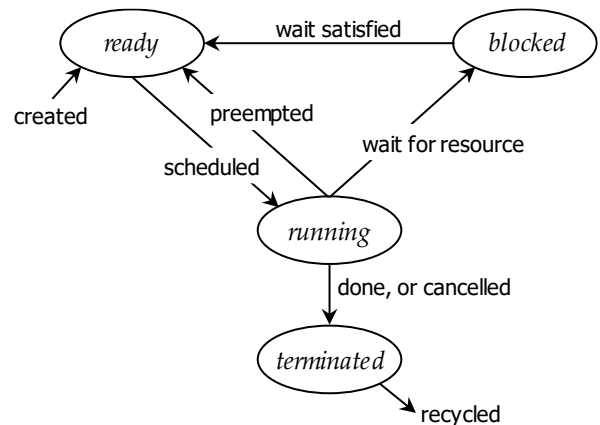
Figure 3. State transitions for a thread.
