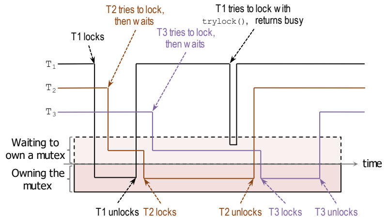
Figure 4. Mutex operation on 3 threads (T 1 , T 2 , T 3 ).
