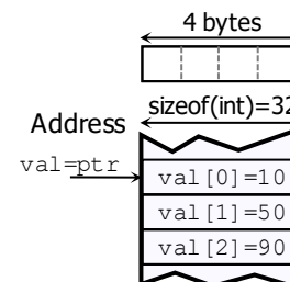
Figure 2. Array after the program executes. sizeof(int) = 32 bits .
