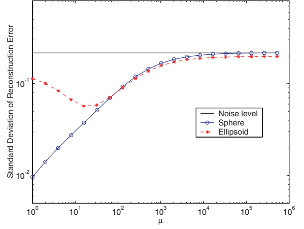
Figure 2. Standard deviation of reconstruction error vs. regularization parameter \alpha = 1/\mu for different shapes.
