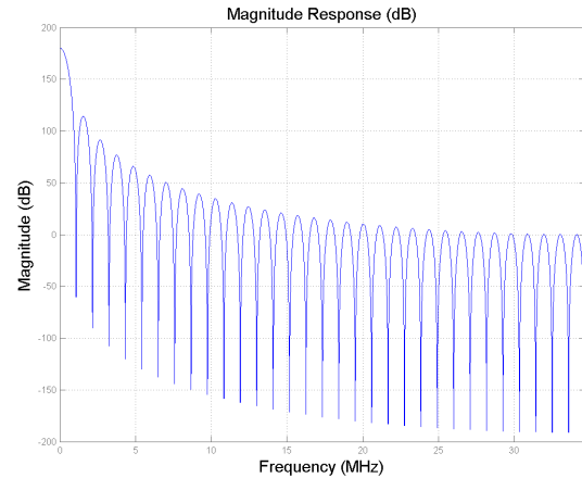
Figure 48: Magnitude response of 5-stage CIC decimator.
