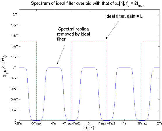
Figure 28: Ideal interpolation filter overlaid with spectrum of sampled signal with f_s = 2f_{\max} .
