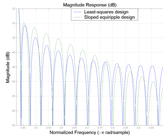
Figure 15: Stopband details of a sloped optimal equiripple FIR design and an optimal least-squares FIR design. The overall error of the equiripple filter approaches that of the least-squares design.
