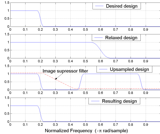
Figure 17: Illustration of the IFIR design paradigm. Two filters are used to attain stringent transition width specifications with reduced total multiplier count when compared to a single filter design.
