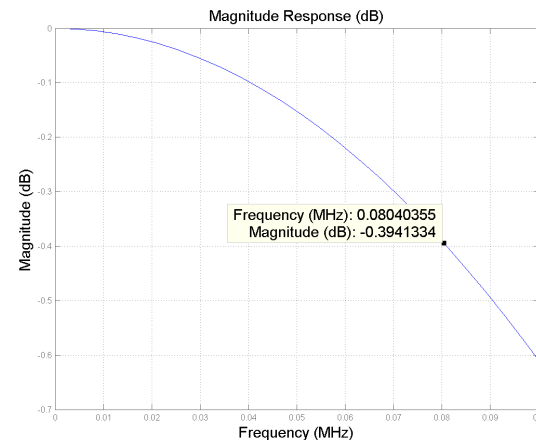
Figure 49: Passband details of scaled 5-stage CIC decimator.
